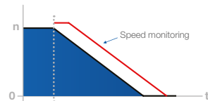
Safe Stop 1 (SS1)
