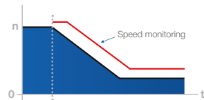
Safely Limited Stop (SLS)
