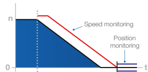
Safe Stop 2 (SS2)
